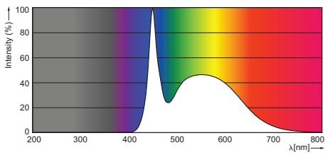
VLE 600 mm 10 W, 1200 mm 20 W /865 T8C Rot
