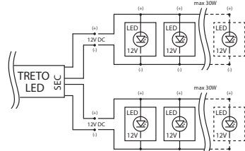
• TRETO LED 30W
